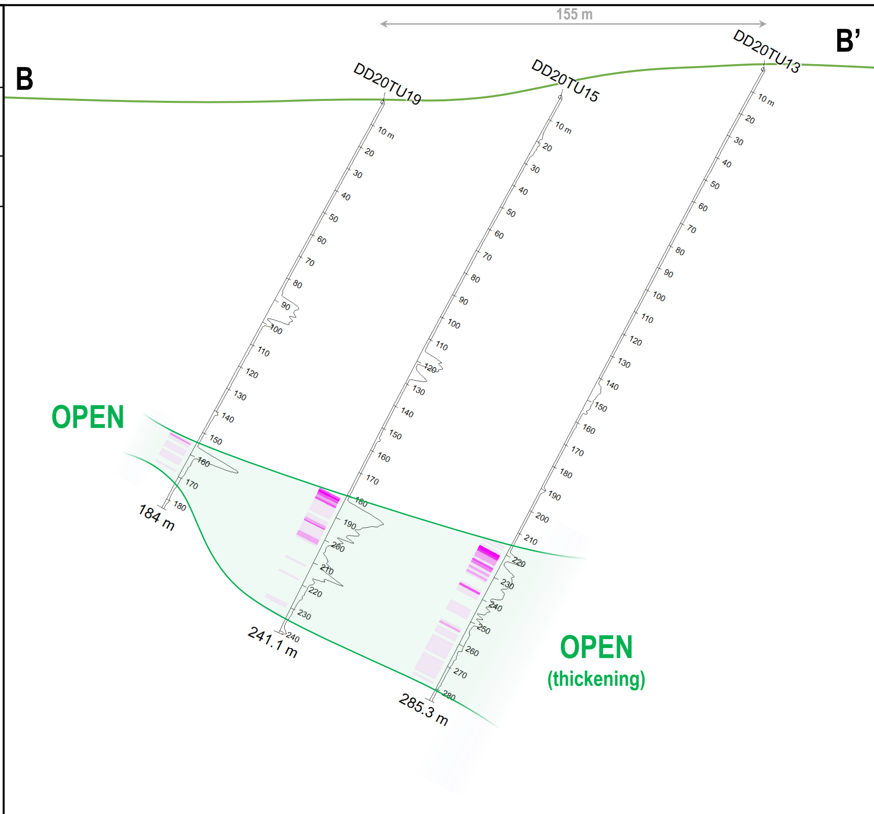
Figure 6: Cross Section of DD20TU15, Up-Dip Hole DD20TU19 and Down-Dip Hole DD20TU13
