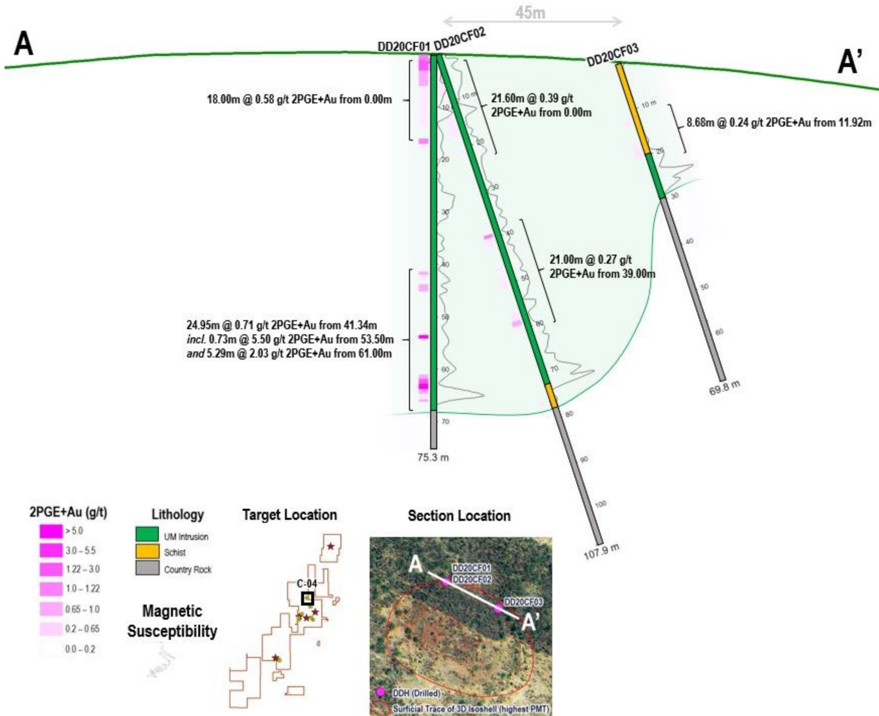
Figure 2: Cross Section of 2020 Drilling at C-04
