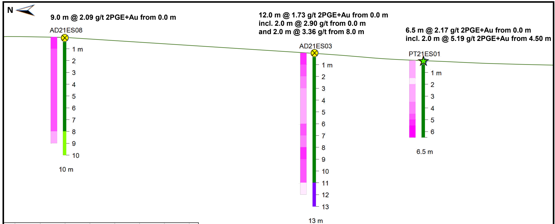
Figure 3: Fence Diagram of Trado Holes ES03 and ES08, and Pit Channel Sample, Esbarro NW Target
