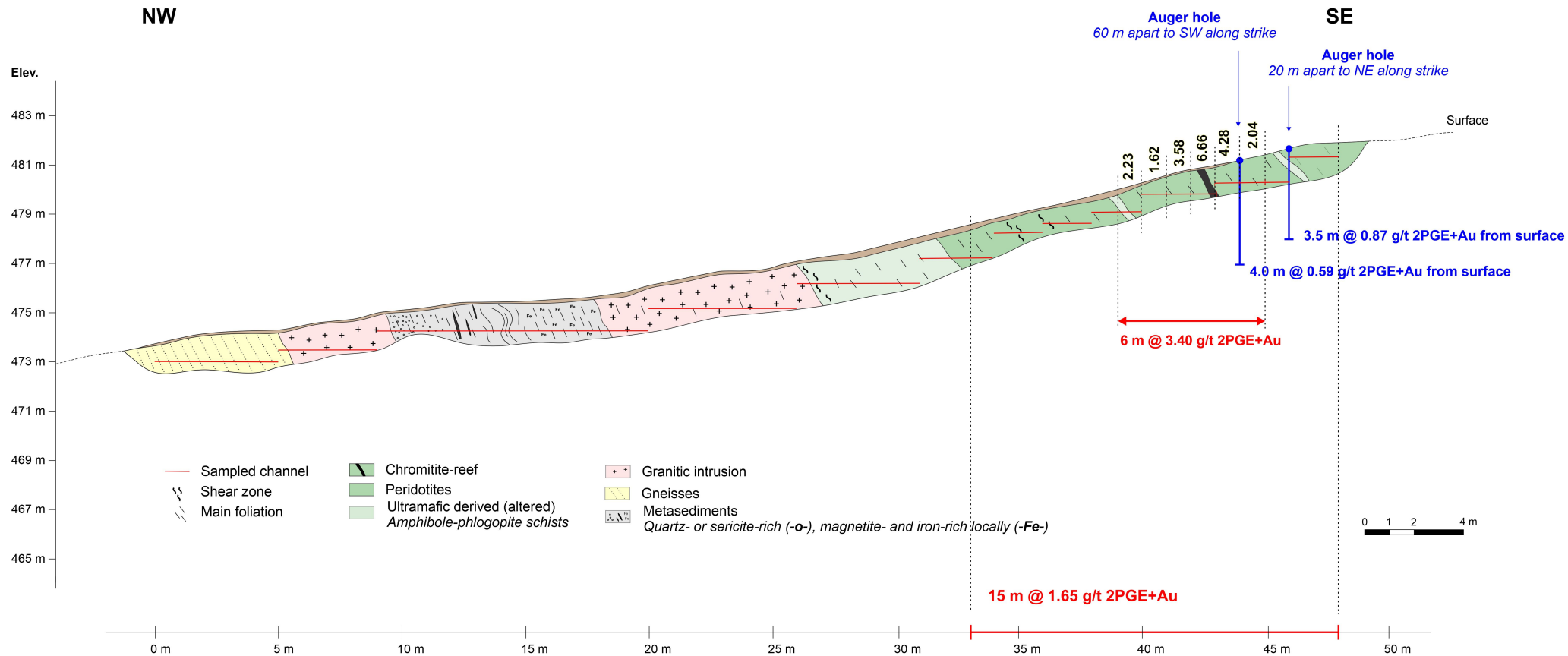
Figure 3c: Trench TR21MS05 Cross Section
