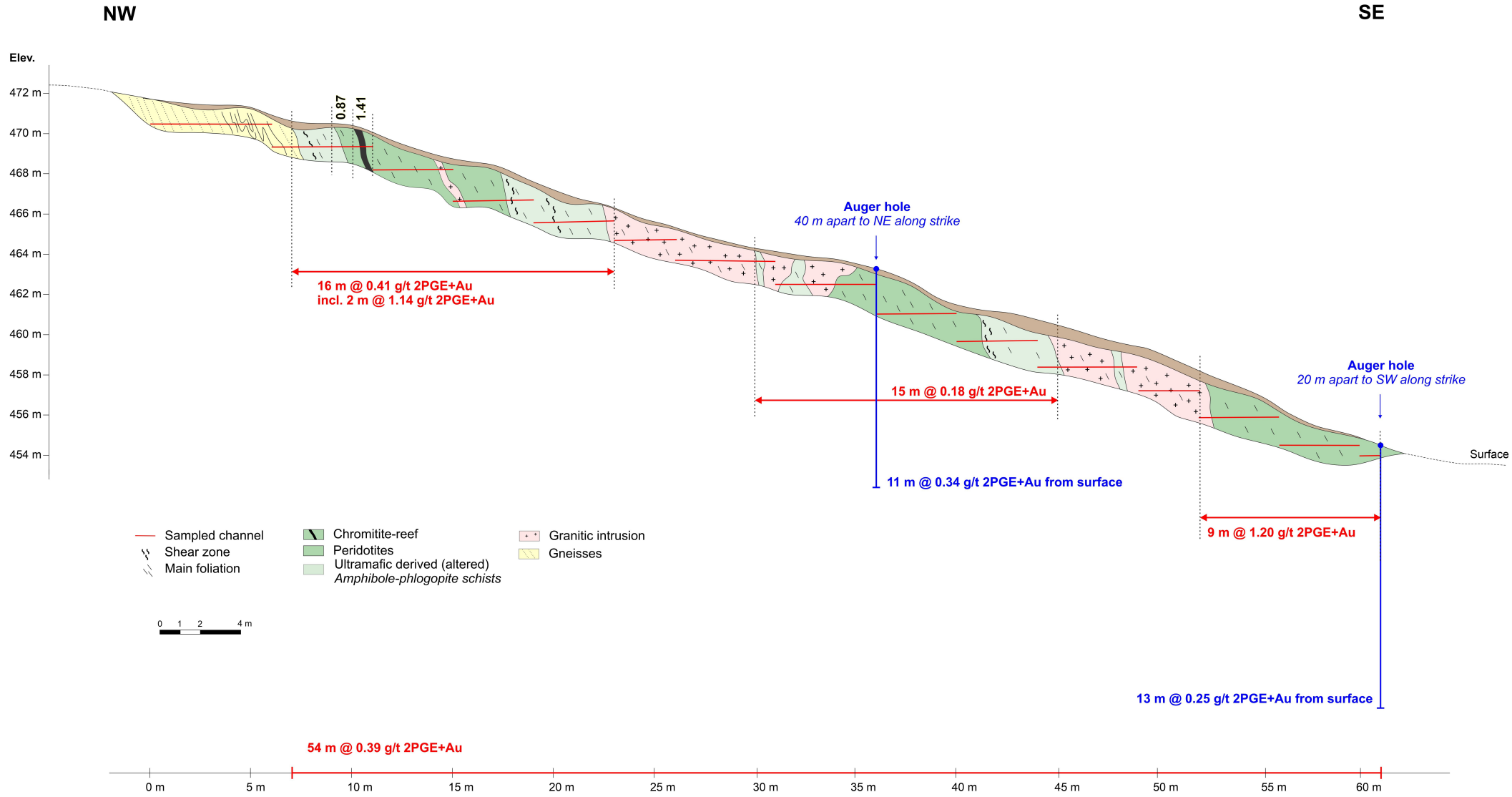
Figure 3a: Trench TR21MS03 Cross Section
