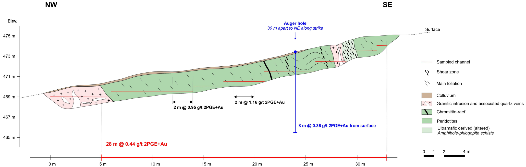
Figure 3b: Trench TR21MS04 Cross Section
