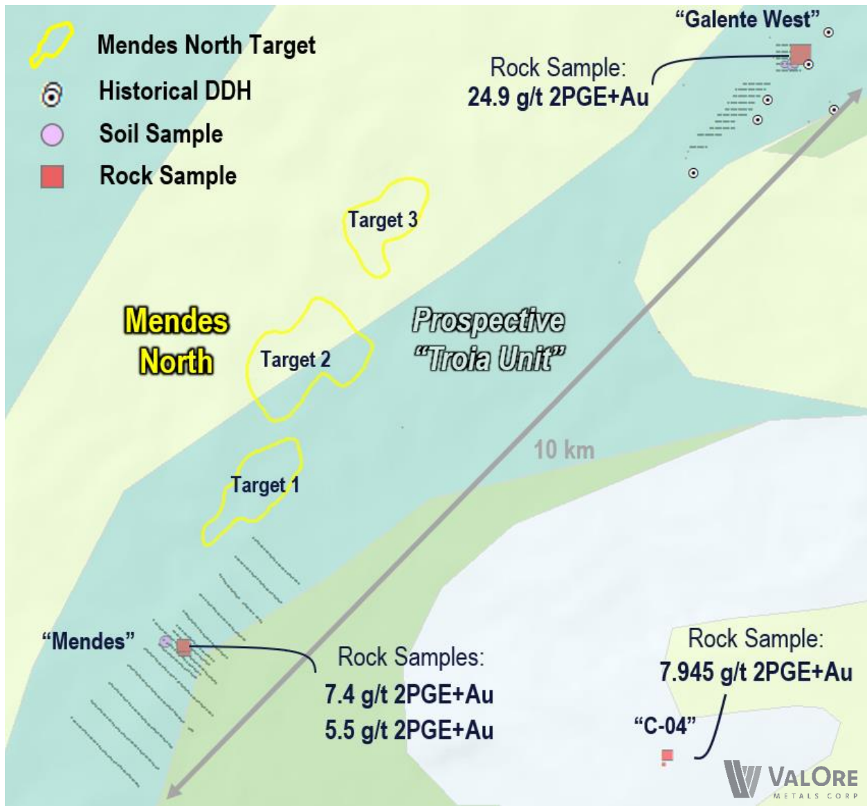
Figure 1: Regional Setting of Mendes North PGE+Au Targets
