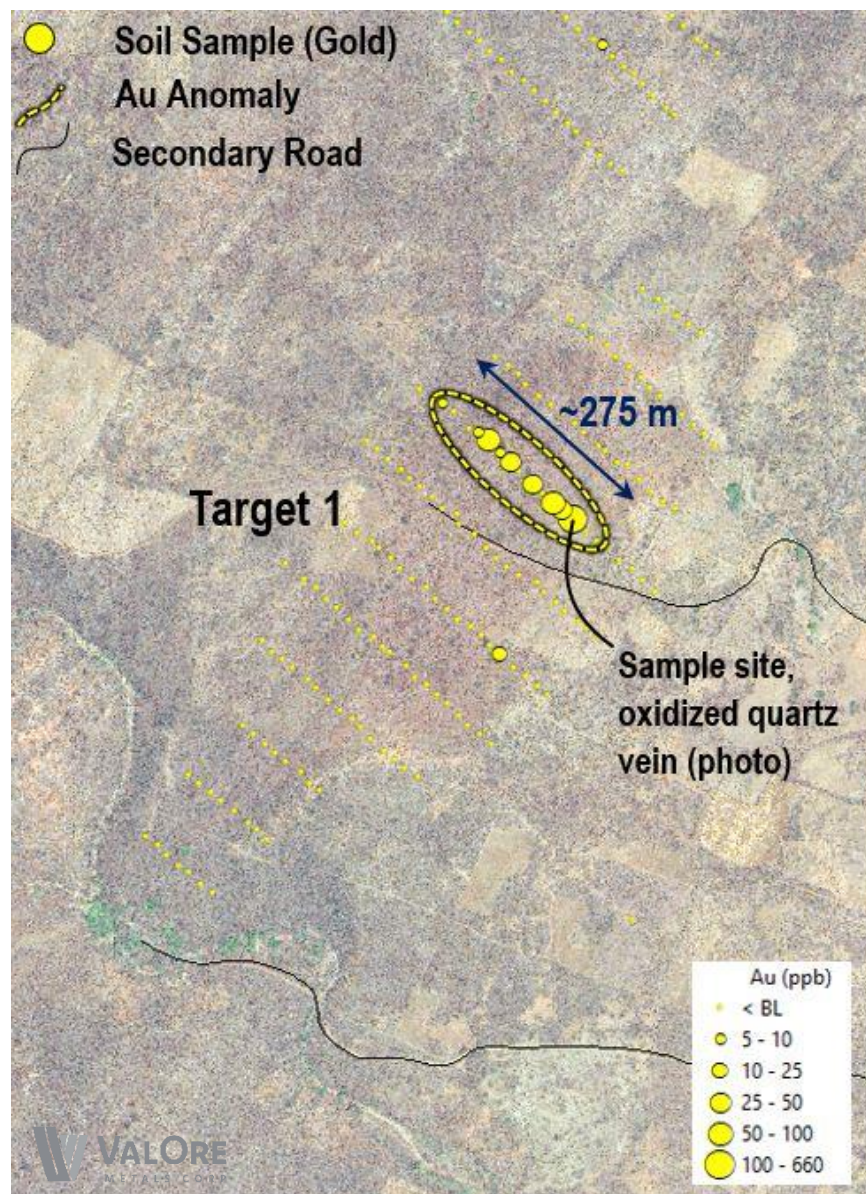
Figure 5: Mendes North Target 1 Gold Anomaly
