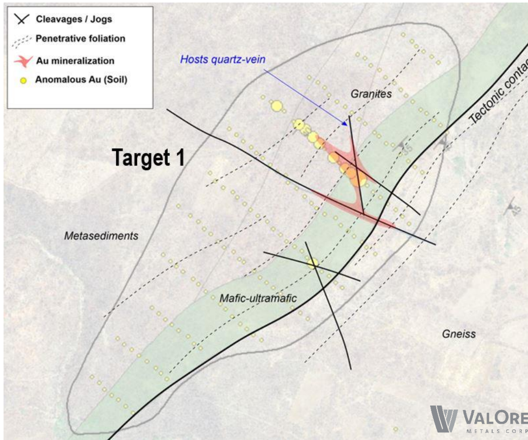
Figure 6: Mendes North Target 1 Gold Anomaly Preliminary Interpretation
