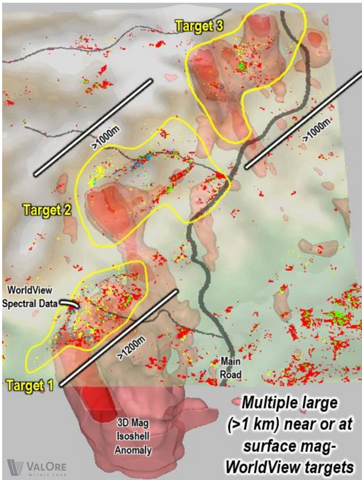
Figure 2: Mendes North 3D Magnetic Inversion Model and WorldView Spectral Anomalies
