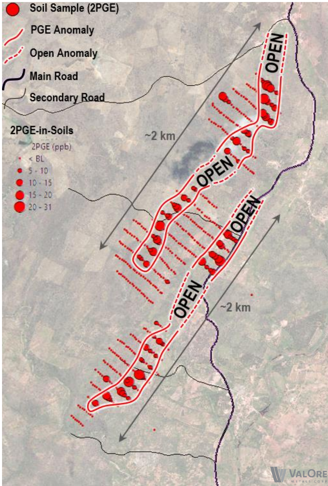
Figure 3: Mendes North PGE-in-Soils Anomalies
